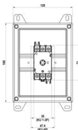
RA2 ENCLOSURE
