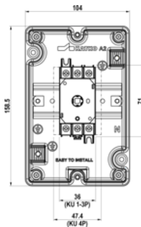
A2 ENCLOSURE
