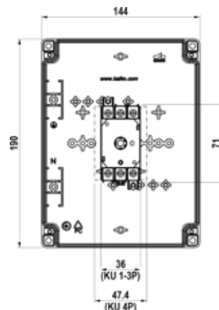
M3 ENCLOSURE
